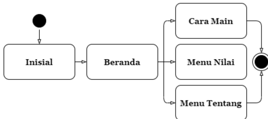
Gambar 3. State Transition Diagram
