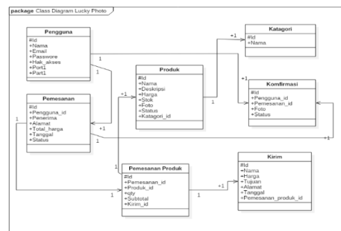
Gambar 6. Class diagram
