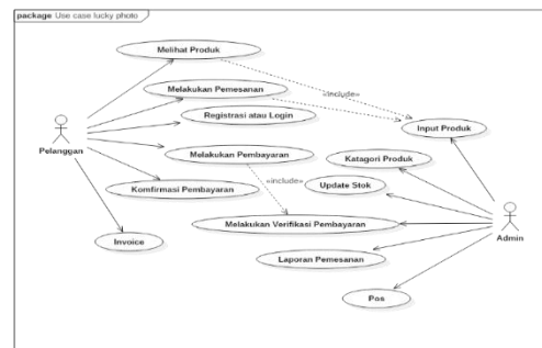
Gambar 5. Use Case diagram
