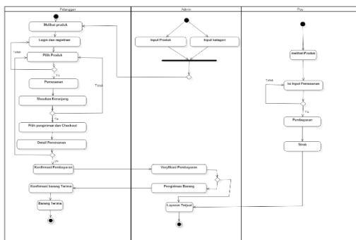
Gambar 4. Activity diagram
