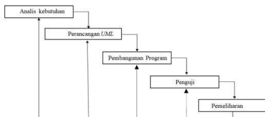
Gambar 1. Metode Waterfall
